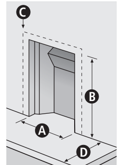
Fireplace dimensions for ALL models
