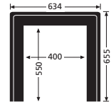
Optional inset steel fitting frame
