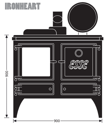
Fireplace dimensions for ALL models
